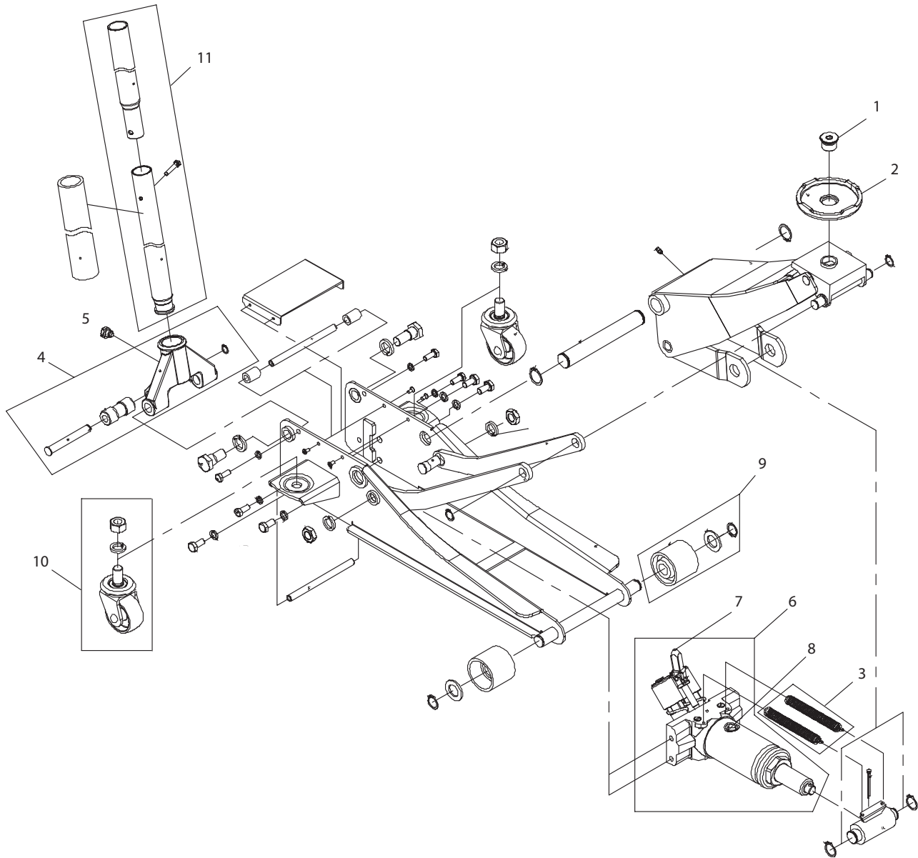
Figure 2 - Replacement Parts Illustration for Model 29021
