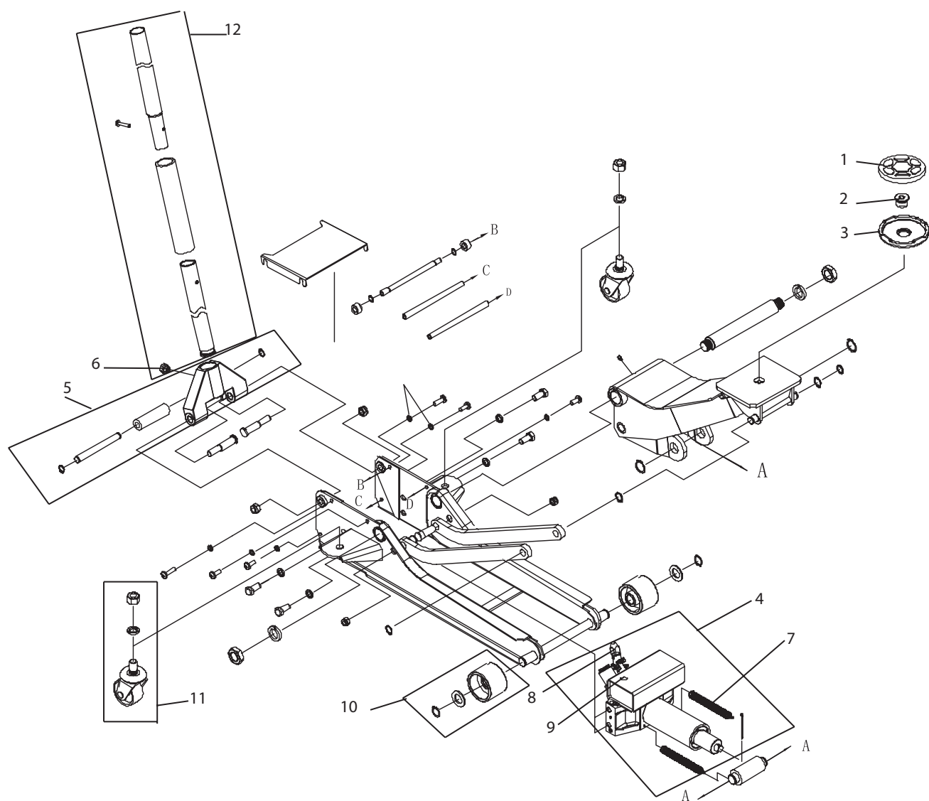
Figure 5 - Replacement Parts Illustration for Model 29033.
